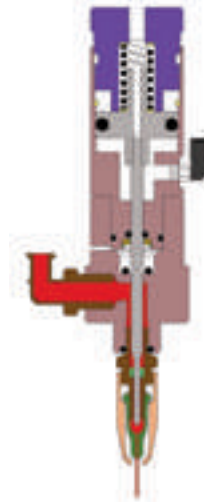
TS5440 Microshot Needle Valve
