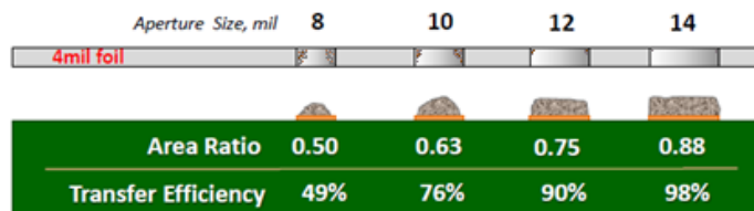
Figure 1 – Examples of expected transfer efficiencies for different aperture area ratios 4 .
