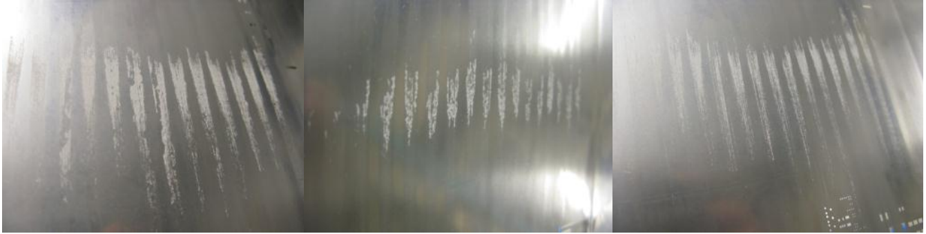
Figure 21 – Remaining solder paste after the first cleaning cycle, A (left), B (middle) and C (right).
