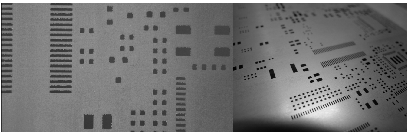
Figure 12 – Example of result after ordinary under stencil cleaning for one of the tested cleaning papers.
