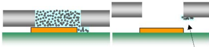
Figure 3 – Smearred solder paste under stencil 5 .
